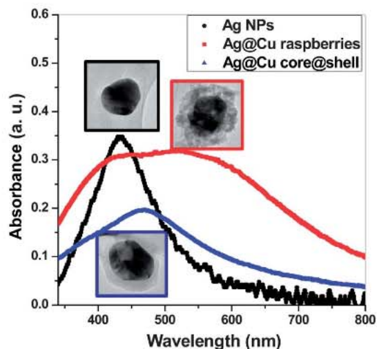
Fig. 2 Comparison of UV-Vis absorption spectra of the Ag nanoparticles and the Ag@Cu bimetal nanoparticles with a raspberry-like or a core@shell nanostructure.
