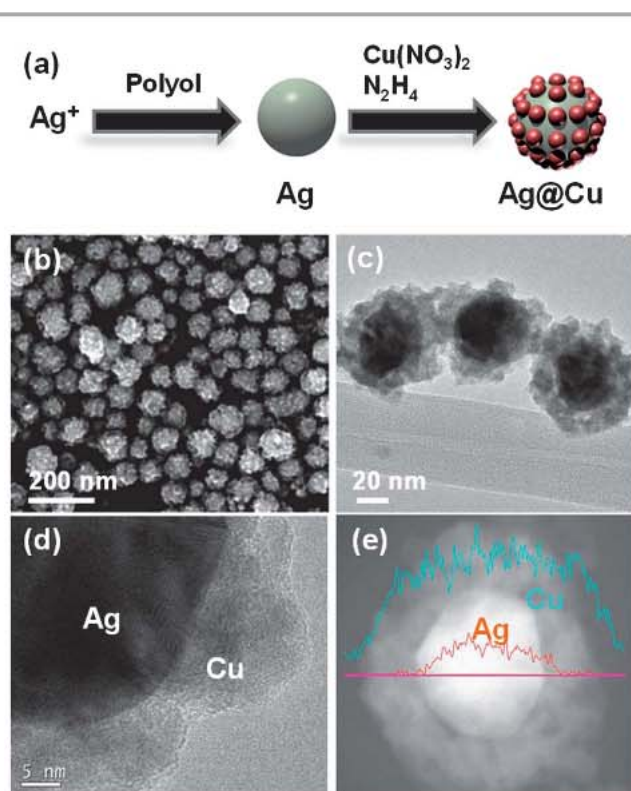
Fig. 1 (a) Scheme of fabrication of the raspberry-like Ag@Cu bimetal nanoparticles and structure analyses of the raspberry-like Ag@Cu bimetal nanoparticles. (b) SEM image of Ag@Cu particles loaded on a silicon substrate, TEM images with low (c) and high (d) magnification, and (e) EDX line-scanning profile across the representative Ag@Cu nanoraspberry bimetal nanoparticles.
